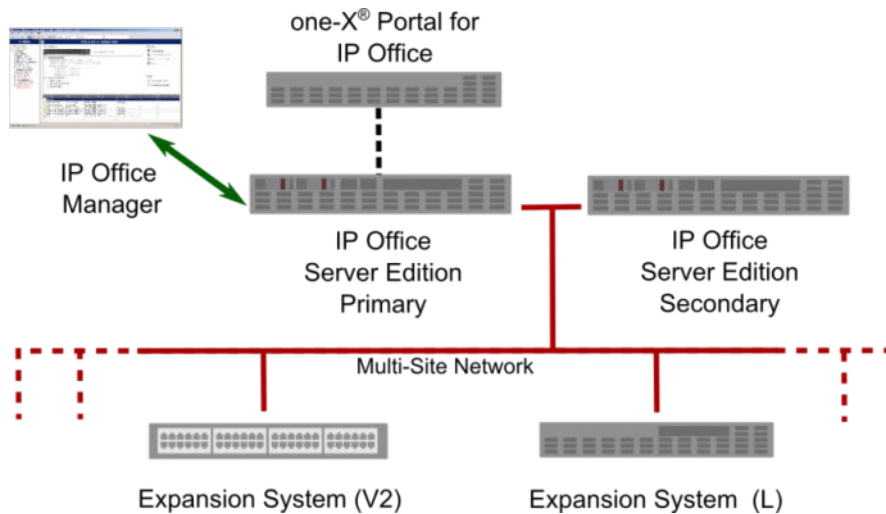
Figure 1: Solution Architecture
